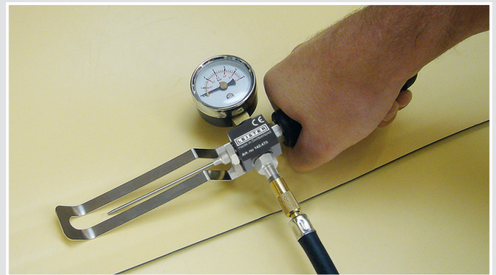
Easy and precise non-destructive seam testing on the construction site
